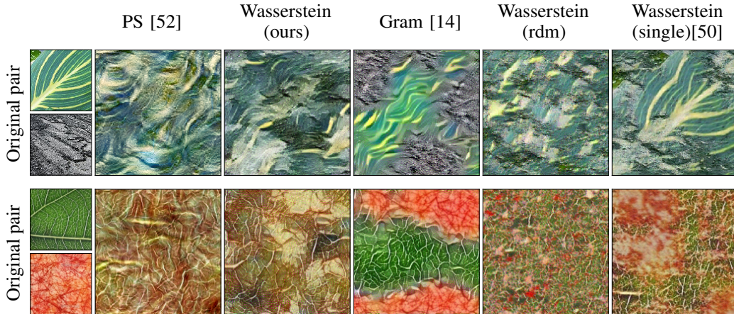
Figure 4: Comparison of textures interpolation methods. PS: the PS algorithm [37] extended to color texture interpolation [52]. Wasserstein (ours), (rdm) and (single): our method eq. (4), using respectively VGG19 pretrained, VGG19 with random weights, and a single layer multiscale architecture [50]. Gram: as in [14] eq. (3). Interpolation weight t = 0.5 .
